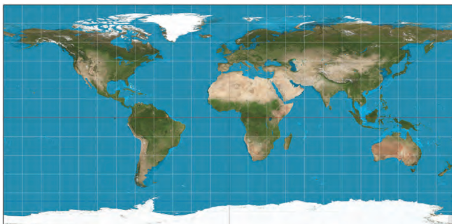
Fig. 14.13: Rectangular map projection
