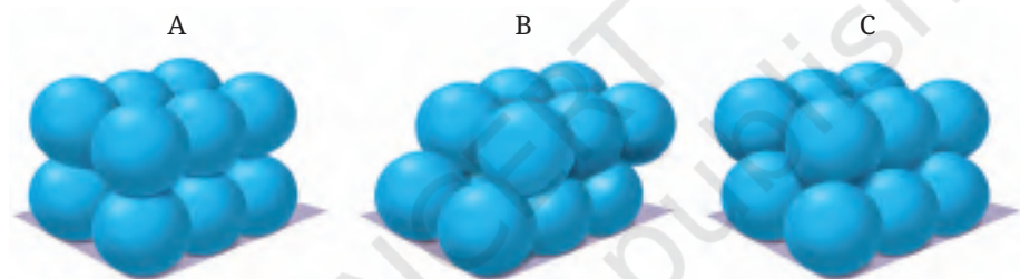
Fig. 14.17: These are some of the ordered ways of packing spheres in a cuboidal structure
