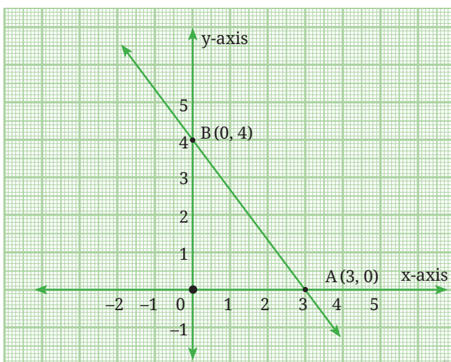
Fig. 13.3: Graph of the linear equation 4x + 3y = 12
