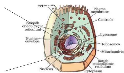
Eukaryotic Cell
